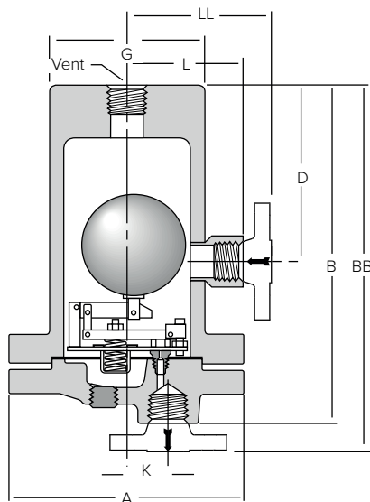
Figure LD-357-1. High leverage ball float drain trap.
