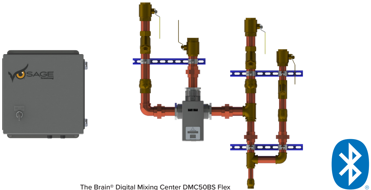
The Brain® Digital Mixing Center DMC50BS Flex
