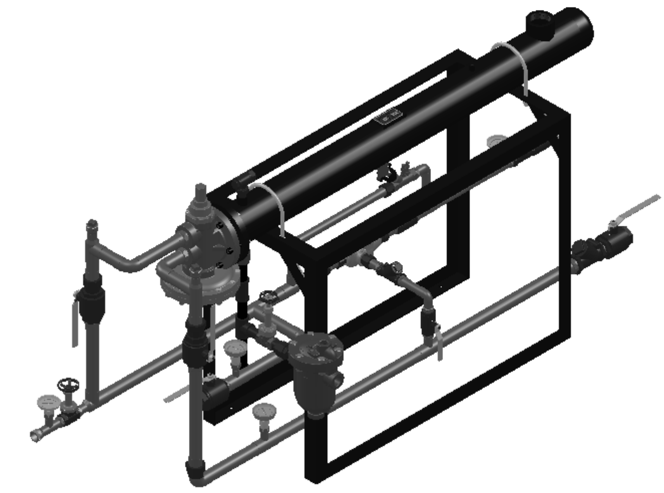
FLO-RITE-TEMP STEAM/WATER HEAT EXCHANGER SINGLE WALL
