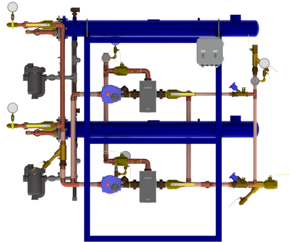
DF535P40-40 Single Wall
