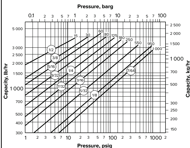
Model 413 Capacity
