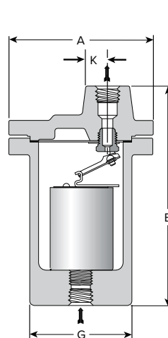
Series 400 Trap
