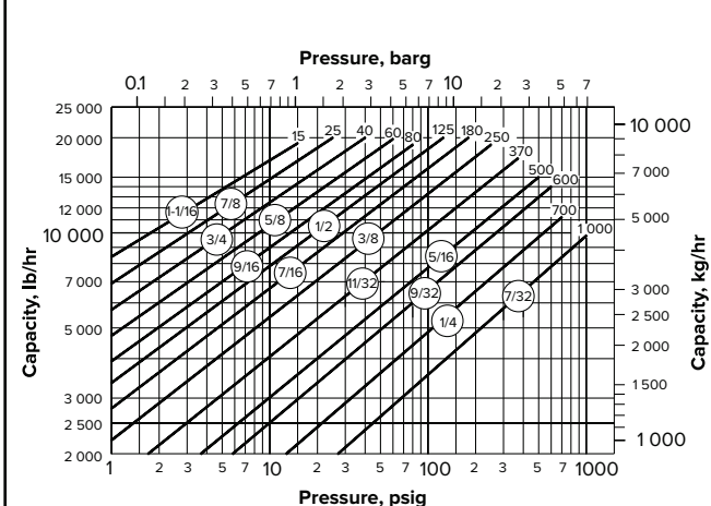
Model 416 Capacity
