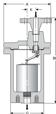
Series 400-FW Trap
