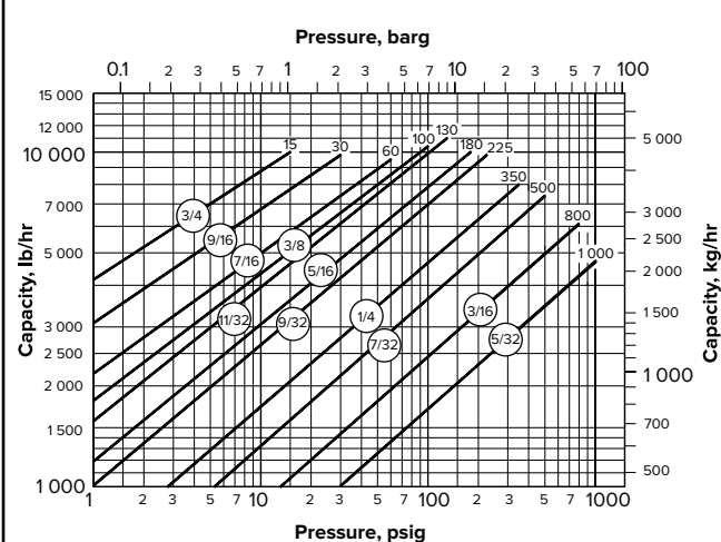
Model 415 Capacity
