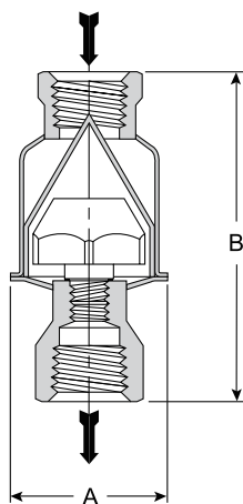
WT-1疏水阀
