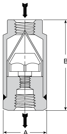
WT-3疏水阀
