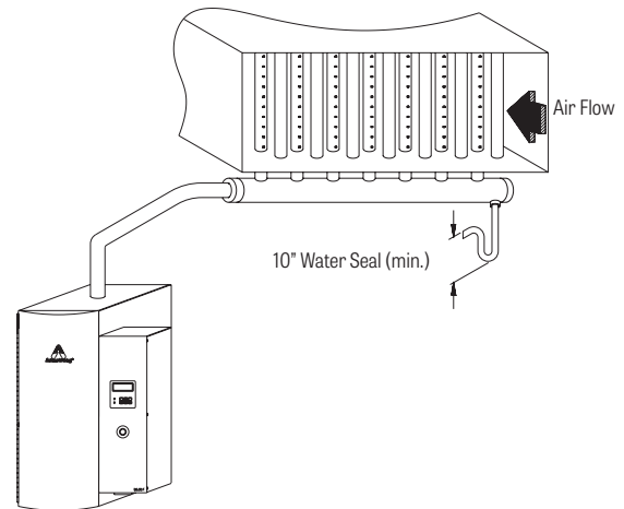
Figure 122-4: HC-6100 or HC-6300 HumidiClean Piped to HumidiPack
