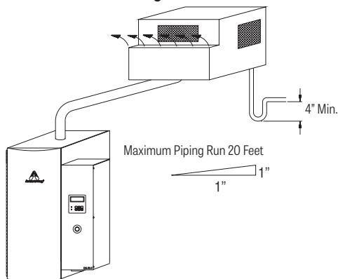
Figure 122-3: HC-6100 or HC-6300 with EHF-3 Fan Package Mounted on Wall
