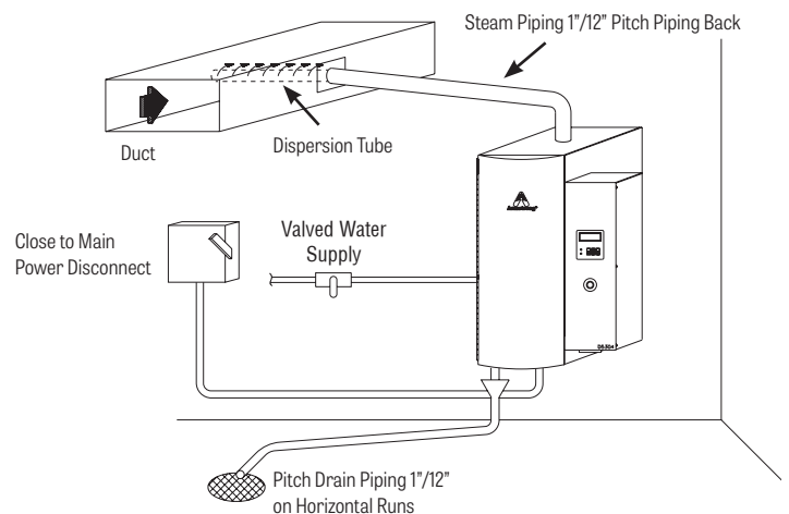
Figure 122-5: HC-6100 or HC-6300 General Installation Concept
