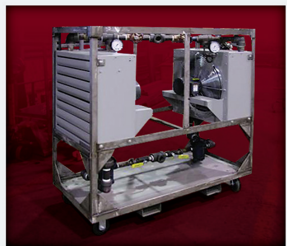
Dual HotBreath™ Heater for Insect Pest Management
