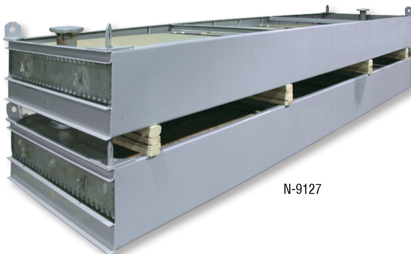
Bare Tube Direct Contact Fluid Bed Dryer Coil
